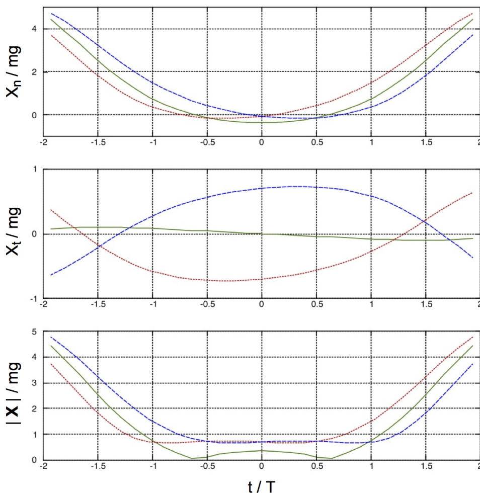
Figure 6. Time dependence of the force \mathbf{X} from the train on the rider, divided by the force of gravity, mg . The normal component X_n is defined as positive in the direction from the seat towards the head of the rider and the tangential force, X_t , is positive in the direction of motion. The third graph shows the absolute value, |\mathbf{X}|/mg . The time has been expressed in terms of the dimensionless quantity T = t/\sqrt{R/g} . The solid curve corresponds to the middle of the train, whereas the dotted and dashed curves give the forces for riders in the front and back of the train. The speed at the top for the middle of the train was chosen to be v_0 = 0.8\sqrt{gR} , resulting in "negative g" on the top.
